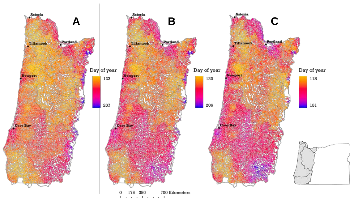
Figure A5.5. Variable infiltration capacity center of flow mass (day of the year) for Western Oregon (Gao et al. 2010), (A) native historical 1930 – 2001, (B) 2040 projection, and (C) 2080 projection. Oregon subset shows the state boundary with the four PS included in this analysis.
